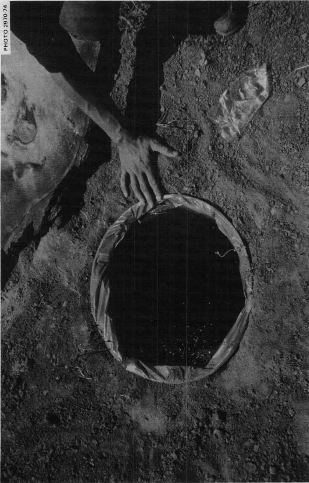
Fig. 4.36. A water storage pit lined with plastic bags, photographed 6 days after having been filled and covered. None of the approximately 25 gallons of water in this pit had leaked through the two 30-gallon trash bags (each about 1\frac{1}{4} mils thick) placed one inside the other for a pit lining.
